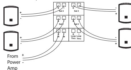
Using Four Control 52 Satellite Loudspeakers
